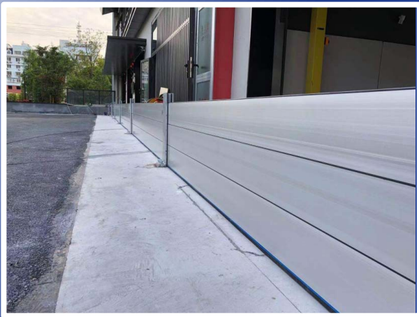
Factory flood protection fence
