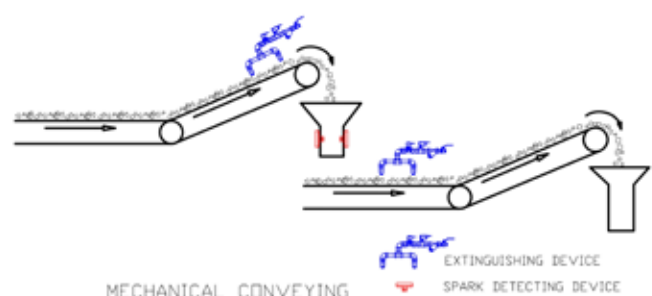
Mechanical conveying
