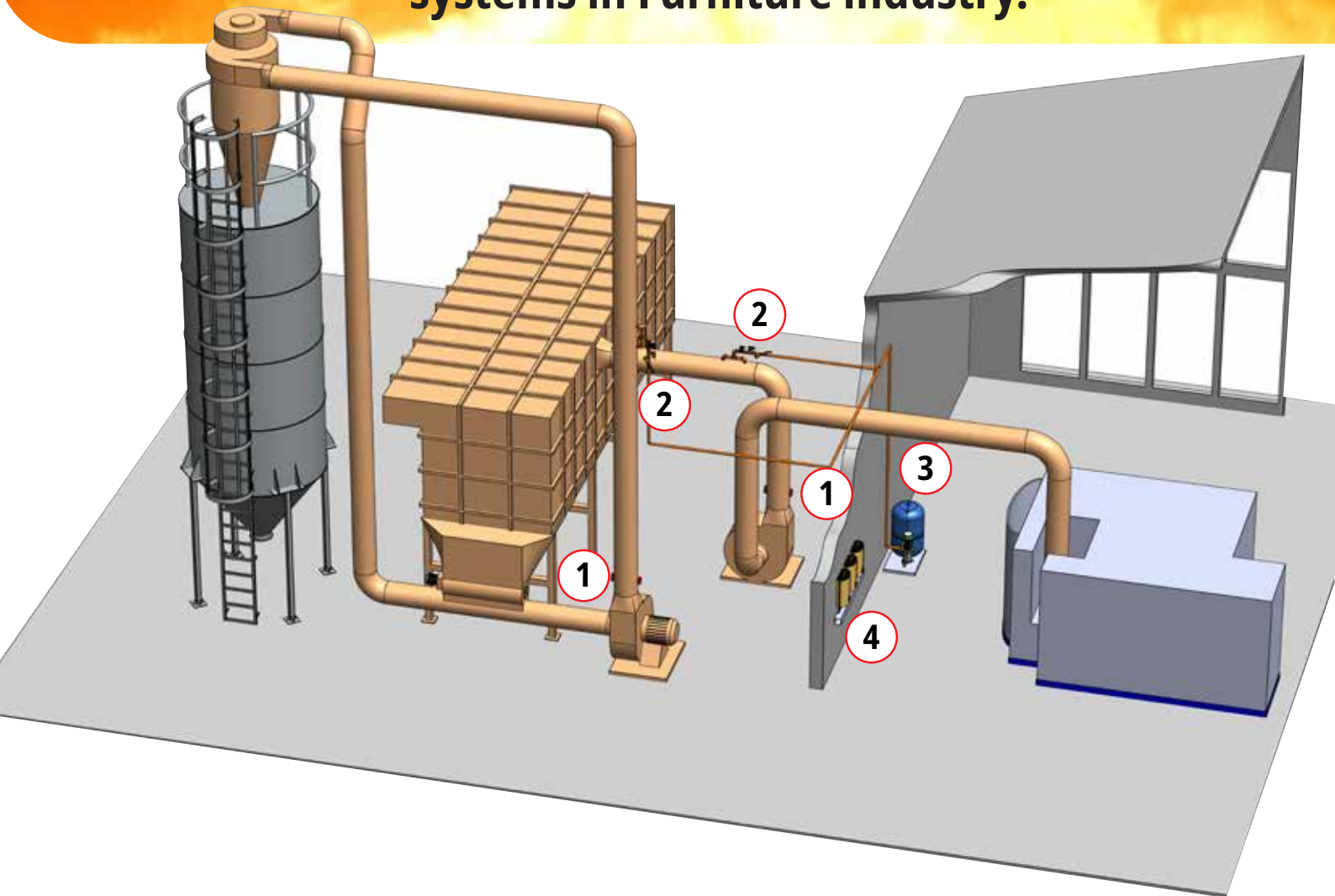
1. Spark Detector
