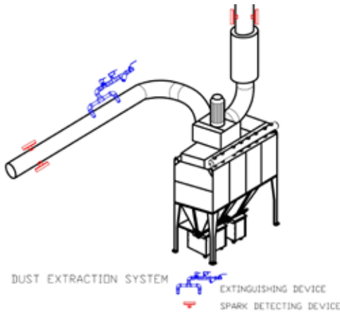
Dust extraction system
