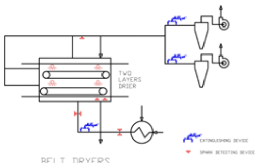
Belt dryers
