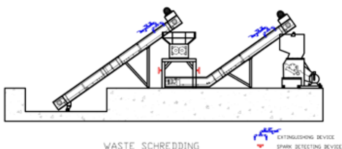
Waste shredding
