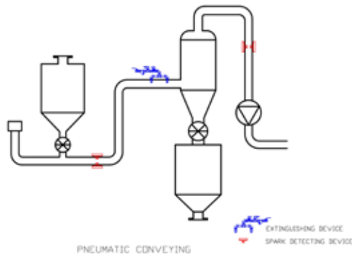
Pneumatic conveying
