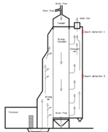
Grain dryer
