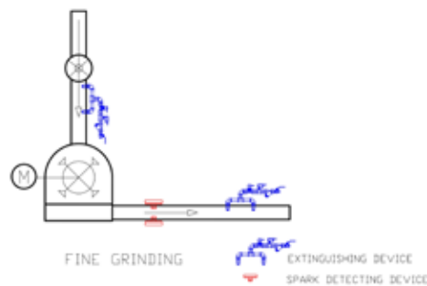
Fine grinding
